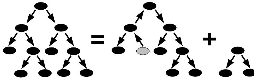
Figure 3.2: Holding a tree as a pair of subtree and its context
