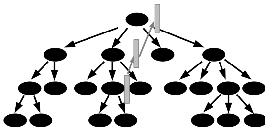
Figure 3.11: Slit for a tree
